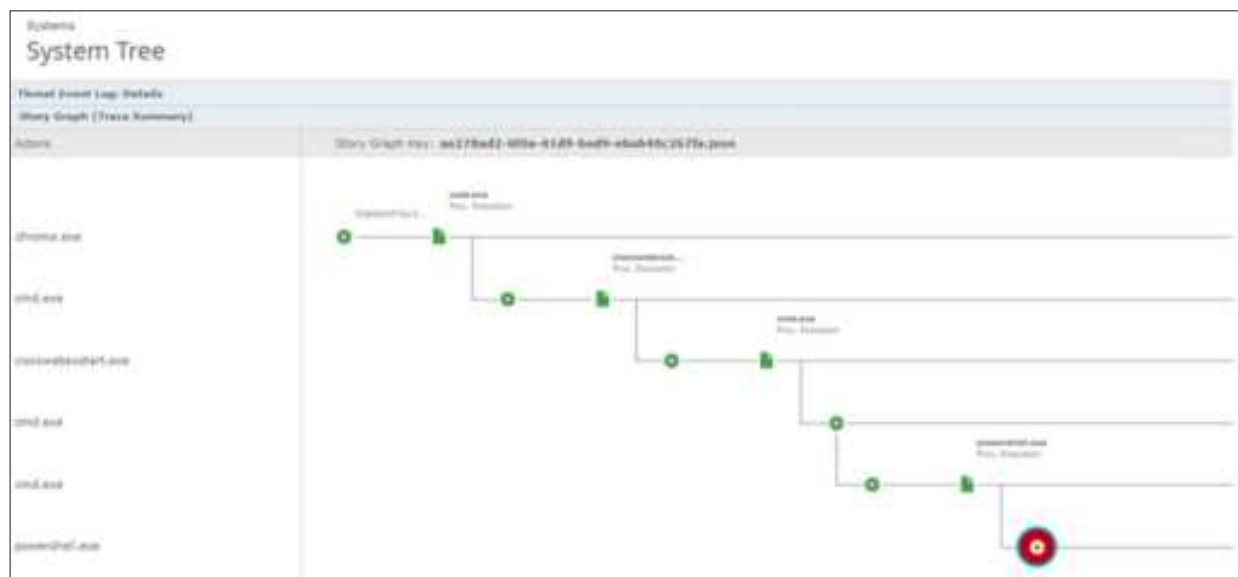
Figure 2. Story Graph
